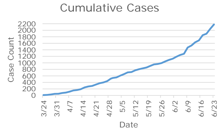
Figure 4: Cumulative number of COVID-19 cases each day.
