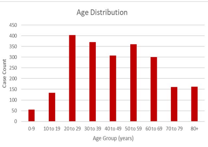
Figure 2: Age of reported COVID-19 cases in PHR 7.
